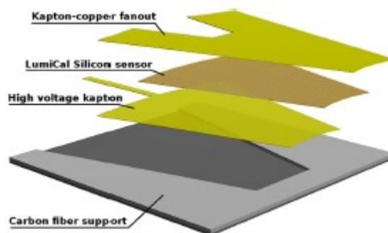
Fig. 2 Detector plane assembly. Total thickness is 650 \mu\text{m}
