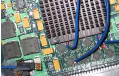
FIGURE 4-53: Wired Prototype
