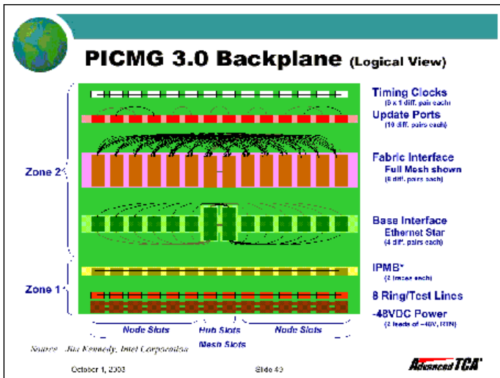
FIGURE 4-3: PICMG 3.0 Backplane
