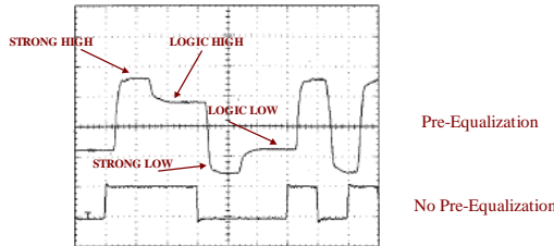
FIGURE 3-26: Pre-Emphasis
