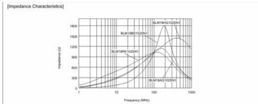
FIGURE 4-14: Sample Impedance Plots
